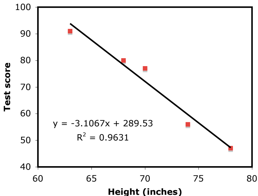
Figure 33. Least-squares fit to data on test score vs. height for a hypothetical class
