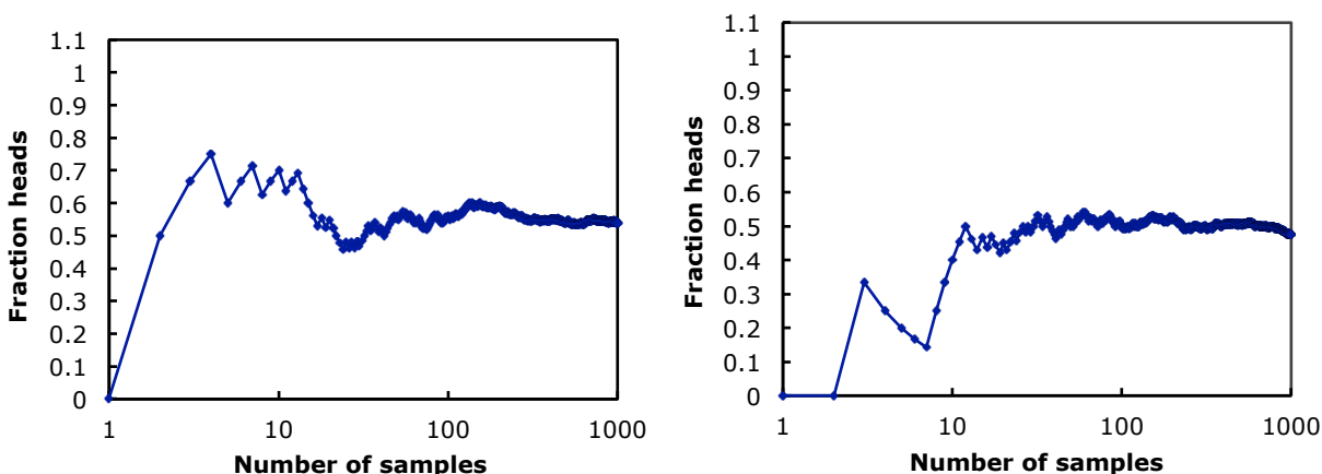
Figure 32. Results of two coin-toss experiments.
