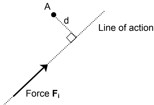
Figure 3. Force, line of action and moment of force ( = Fd ) about a point A. The example shown is a counterclockwise moment of force, i.e. force F_i is trying to rotate the line segment d counterclockwise about point A.
