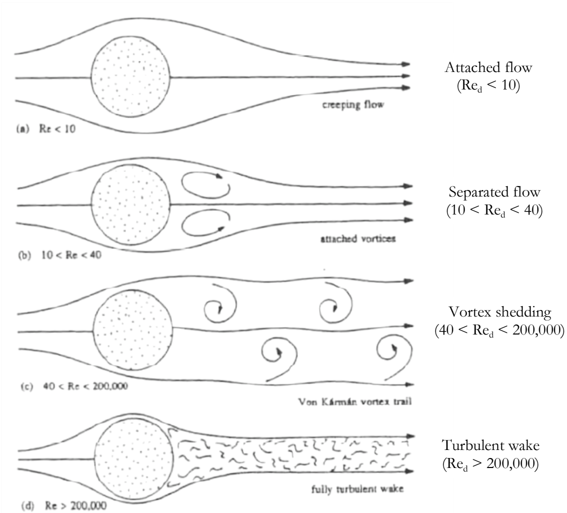
Figure 19. Schematic of flow around a cylinder at different Reynolds numbers
